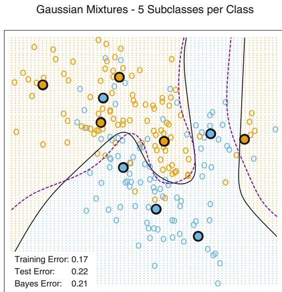
FIGURE 13.2. The upper panel shows the K-means classifier applied to the mixture data example. The decision boundary is piecewise linear. The lower panel shows a Gaussian mixture model with a common covariance for all component Gaussians. The EM algorithm for the mixture model was started at the K-means solution. The broken purple curve in the background is the Bayes decision boundary.
