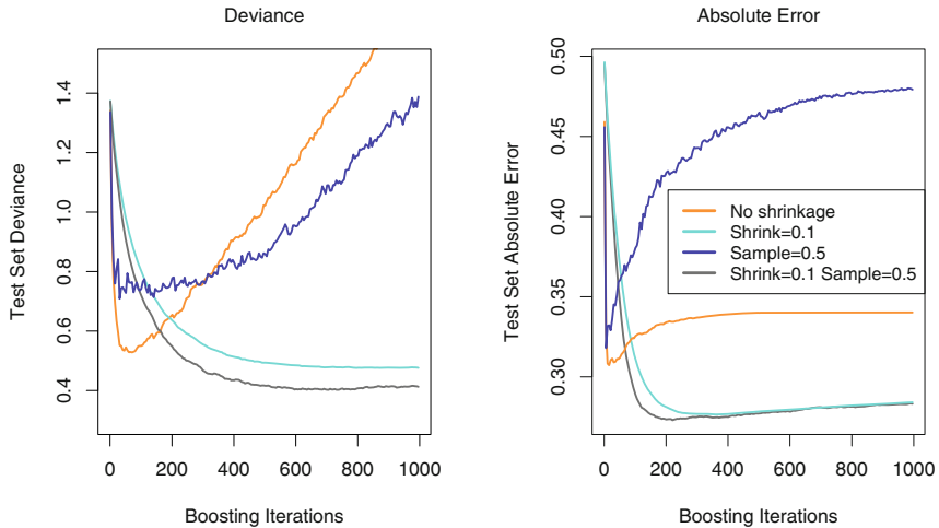
FIGURE 10.12. Test-error curves for the simulated example (10.2), showing the effect of stochasticity. For the curves labeled “Sample=0.5”, a different 50% subsample of the training data was used each time a tree was grown. In the left panel the models were fit by gbm using a binomial deviance loss function; in the right-hand panel using square-error loss.
